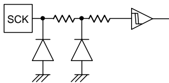
Figure 47. SCK input equivalent circuit
