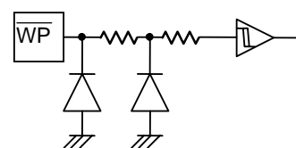
Figure 50. \overline{WP} input equivalent circuit
