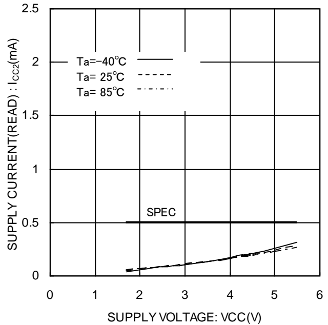
Figure 15. Supply current (READ) I_{CC2}(\text{READ}, f_{SK}=1\text{MHz})
