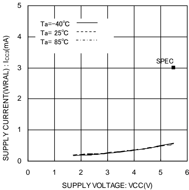
Figure 18. Supply current (WRAL) I_{cc3} (WRAL, f_{sk}=3\text{MHz} )
