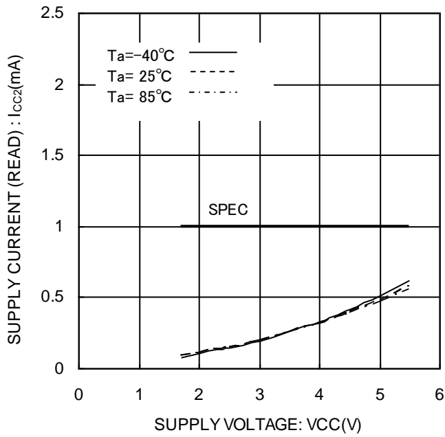
Figure 16. Supply current (READ) I_{cc2} (READ, f_{sk}=3\text{MHz} )
