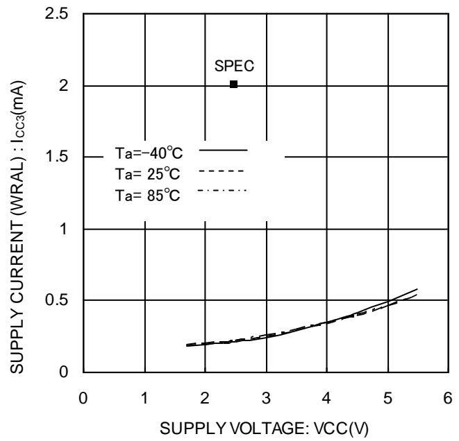
Figure 17. Supply current (WRAL) I_{cc3} [WRAL, f_{sk}=1\text{MHz} ]
