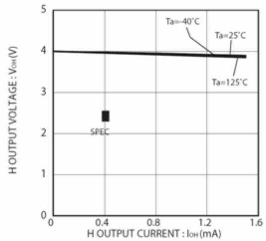
Figure 6. H output voltage V_{OH} - I_{OH} ( V_{CC}=4.0V )
