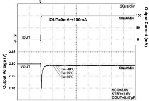
Fig 195. Load Response
