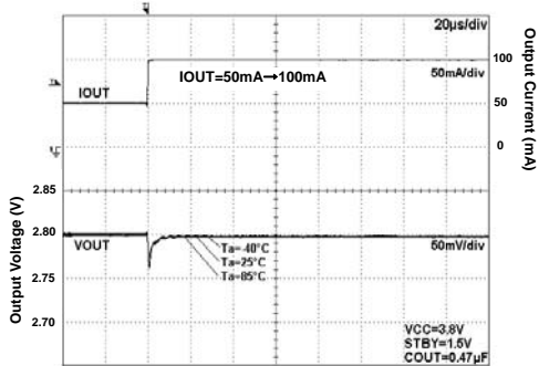
Fig 199. Load Response
