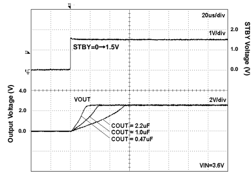
Fig 150. Start Up Time Iout=200mA
