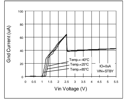
Fig. 65 Circuit Current IGND
