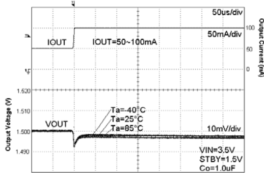
Fig. 22 Load Response
