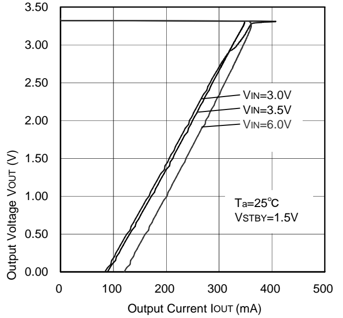
Figure 75. OCP Threshold
