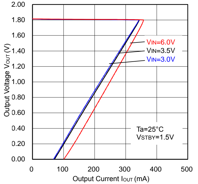
Figure 8. OCP Threshold
