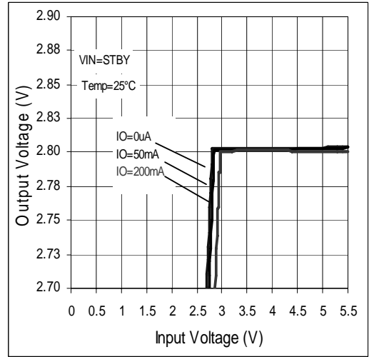
Figure 27. Line Regulation
