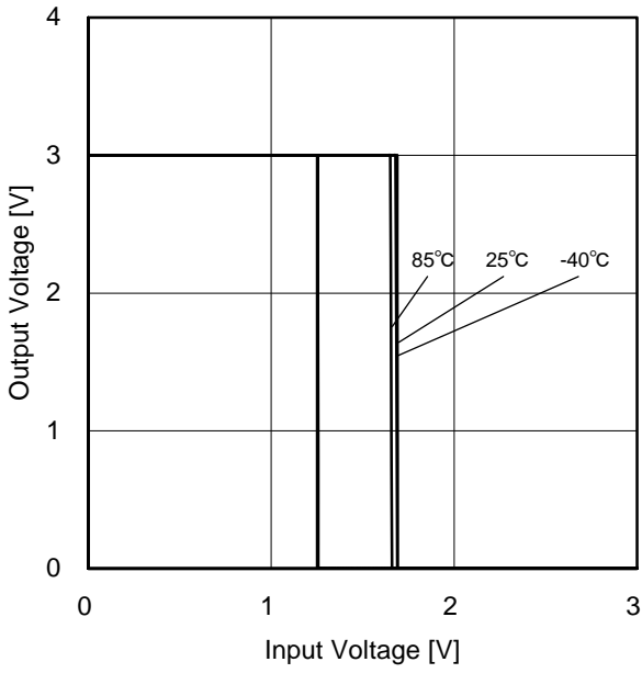
Figure 1. Output Voltage vs Input Voltage (V DD =3V / V SS =0V)
