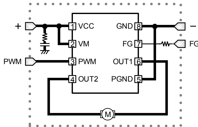
Figure 1. Application circuit
