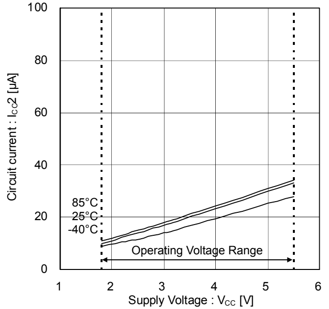
Figure 4. Circuit Current 2 (Stand-by mode)
