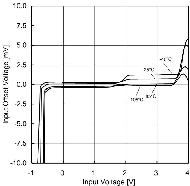
Figure 39. Input Offset Voltage vs Input Voltage ( V_{DD}=3V )
