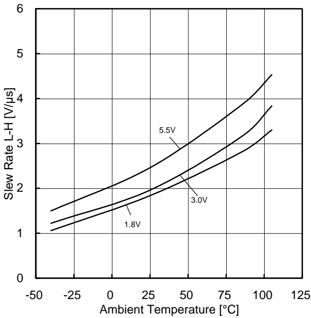
Figure 68. Slew Rate L-H vs Ambient Temperature
