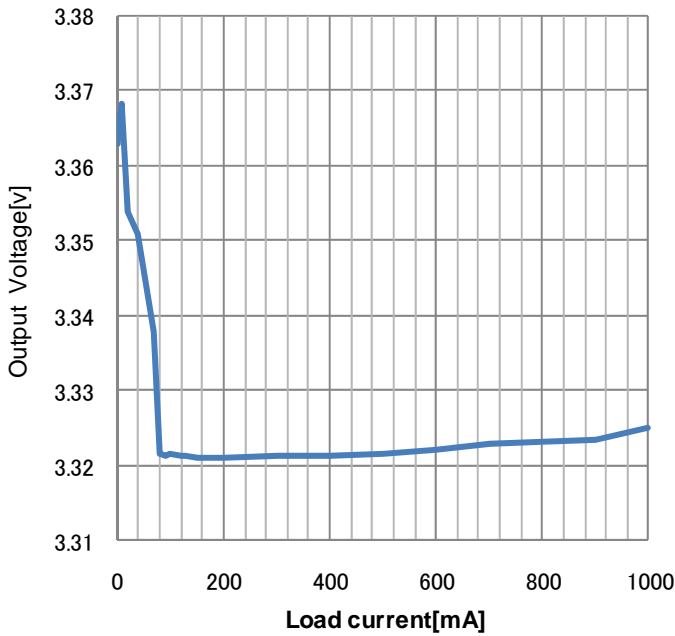
Figure 15. Load regulation VIN=5V PWM/PFM Auto mode
