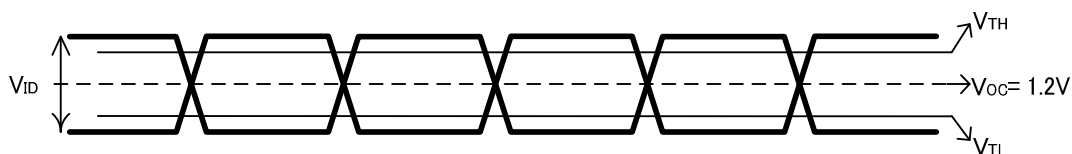
Figure 4. LVDS Receiver DC Specifications
