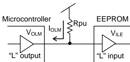
Figure 48. Input terminal pull up resistance
