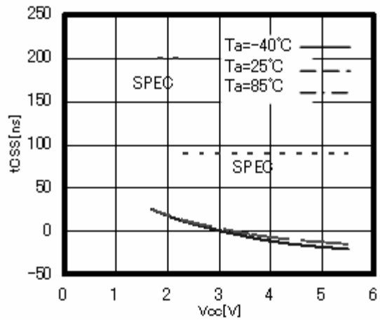
Figure 19. \overline{CS} setup time tCSS
