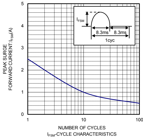
IFSM-CYCLE CHARACTERISTICS
