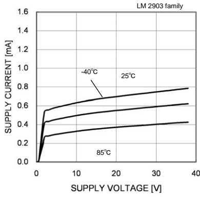
Fig. 42 Supply Current - Supply Voltage
