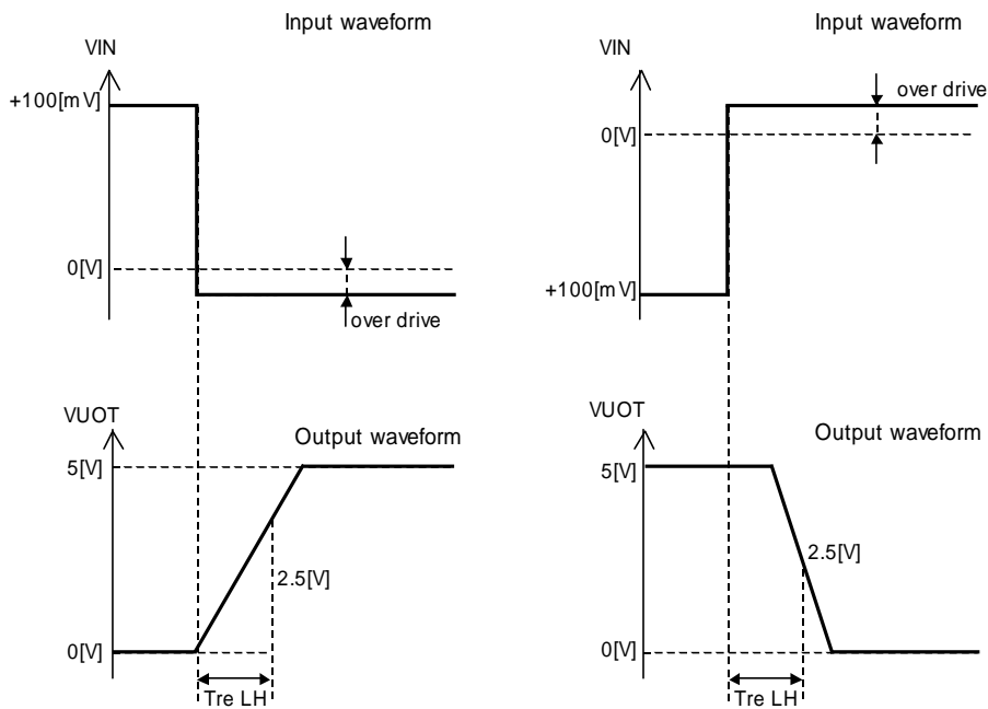
Fig.90 Response Time
