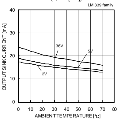
Fig.27 Output Sink Current - Ambient Temperature (VOUT=1.5[V])
