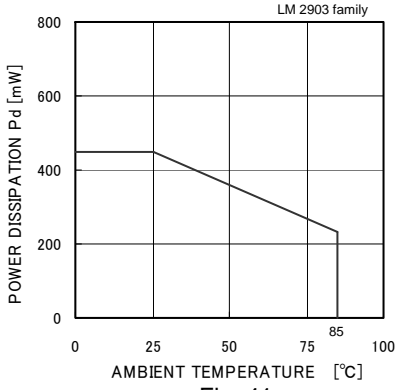
Fig. 41 Derating Curve
