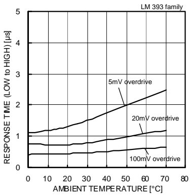
Fig. 19 Response Time (Low to High) – Ambient Temperature (VCC=5[V],VRL=5[V],RL=5.1[kΩ])
