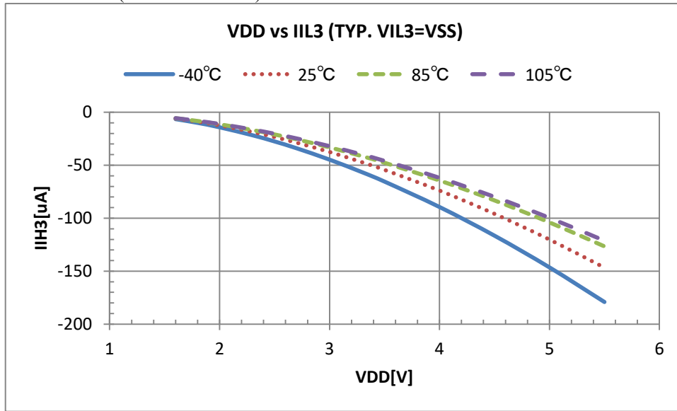
VDD VS IIL3 (TYP. VIL3=VSS)
