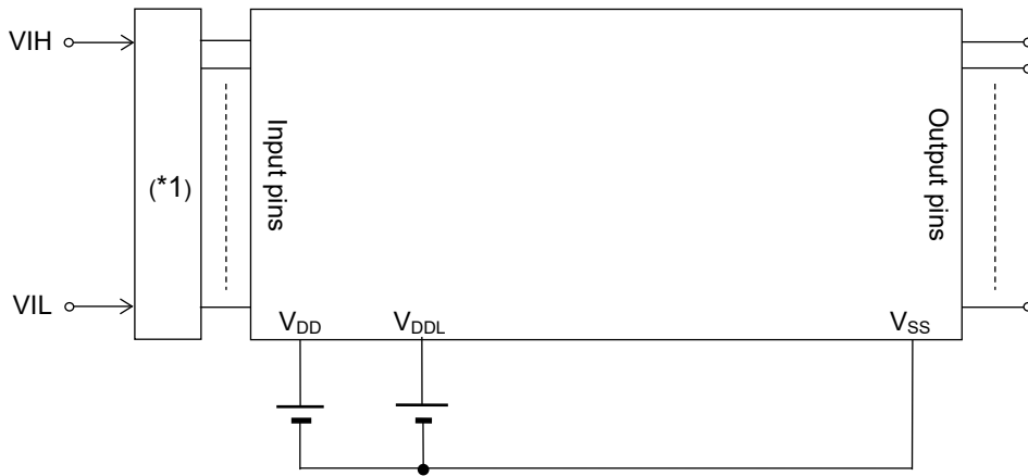
Measuring circuit 5
