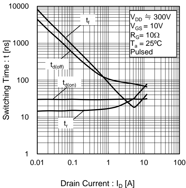
Fig.20 Switching Characteristics
