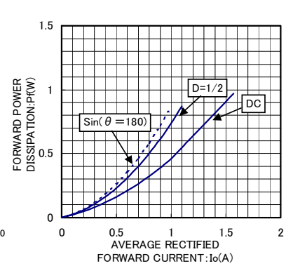
Io-Pf CHARACTERISTICS
