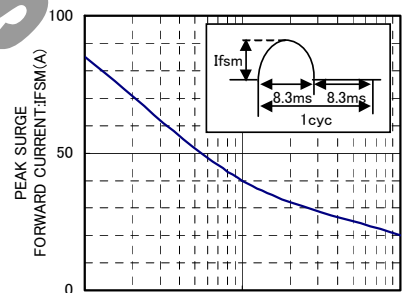
IFSM-CYCLE CHARACTERISTICS
