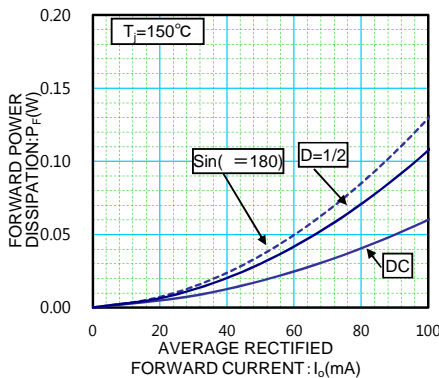
I_o - P_F CHARACTERISTICS
