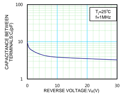
V_R - C_t CHARACTERISTICS
