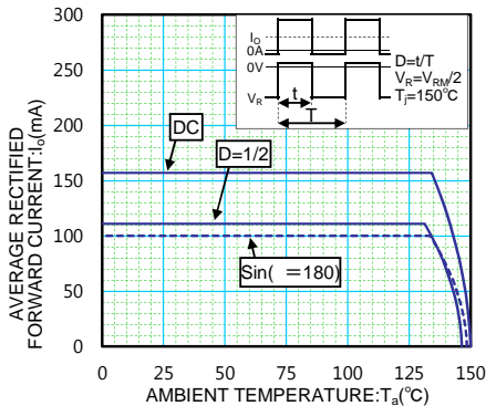
DERATING CURVE ( I_o - T_a )
