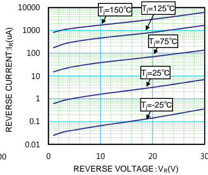
V_R - I_R CHARACTERISTICS
