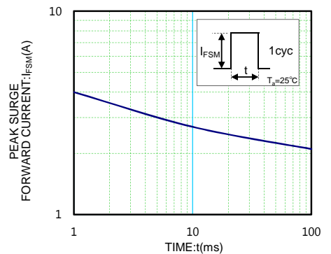
I_{FSM} - t CHARACTERISTICS
