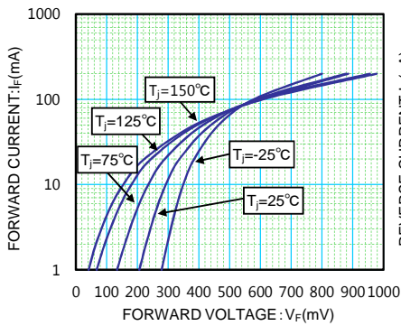
V_F - I_F CHARACTERISTICS
