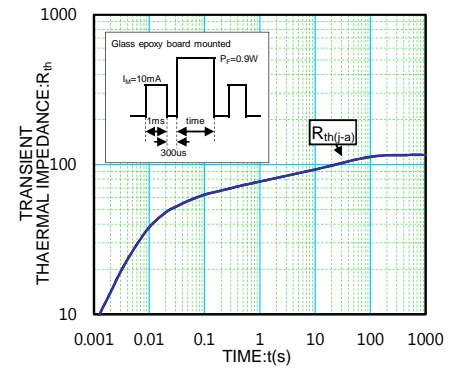
R_{th} - t CHARACTERISTICS
