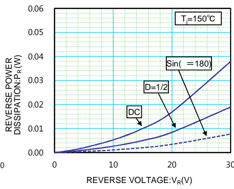
V_R - P_R CHARACTERISTICS
