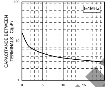
REVERSE VOLTAGE : V_R (V) V_R - C_t CHARACTERISTICS
