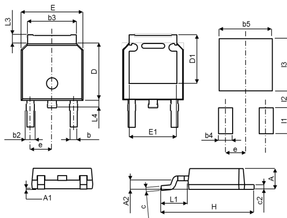
TO-252, (TO-252)
