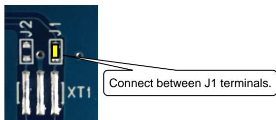
Figure 6 External clock
