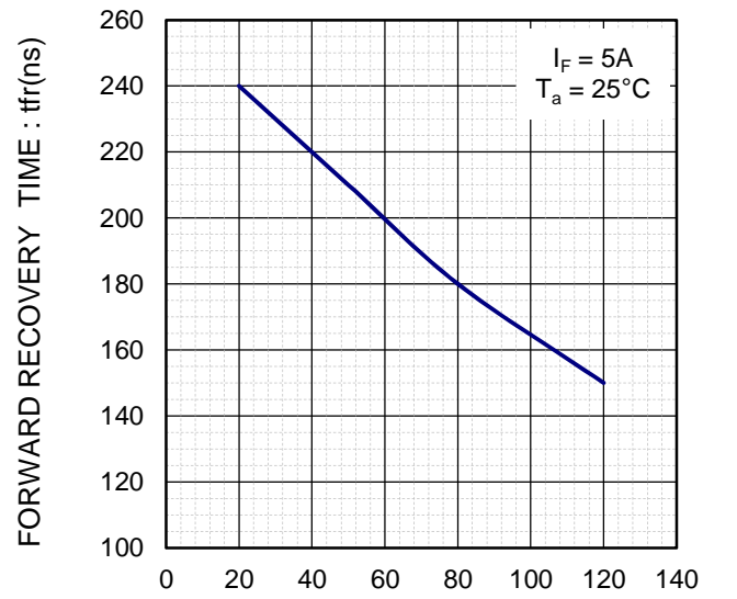
RATE OF CHANGE OF CURRENT : di/dt(A/\mu s) di/dt-t_{fr} CHARACTERISTICS
