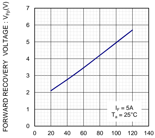
RATE OF CHANGE OF CURRENT : di/dt(A/\mu s) di/dt-V_{FP} CHARACTERISTICS
