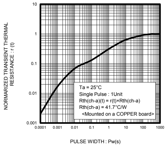
Fig.14 Normalized Transient Thermal Resistance vs. Pulse Width
