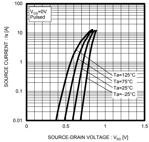
Fig.8 Reverse Drain Current vs. Source-Drain Voltage
