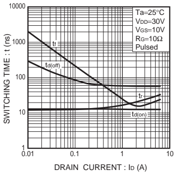
Fig.7 Switching Characteristics
