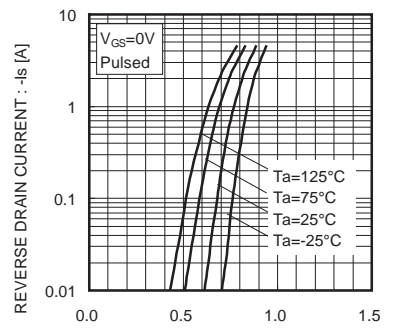
SOURCE-DRAIN VOLTAGE : -V_{SD} [V] Fig.9 Reverse Drain Current vs. Source-Drain Voltage
