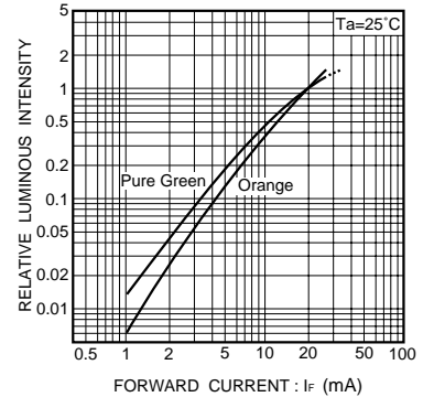
Fig. 31 Luminous intensity vs. forward current
