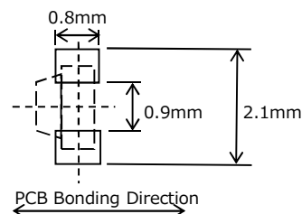
[Sn plated electrode type]
