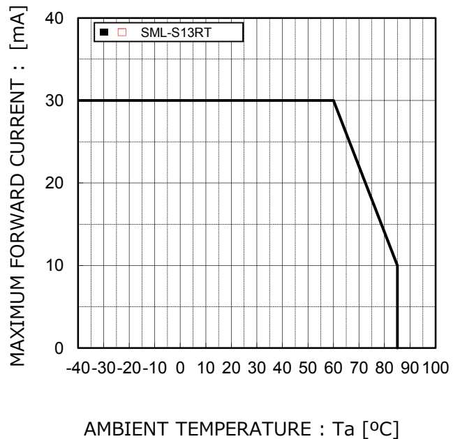
Fig.4 Derating
