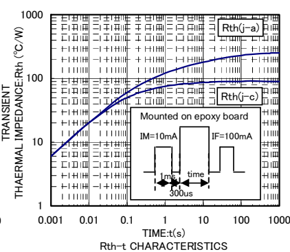
Rth-t CHARACTERISTICS
