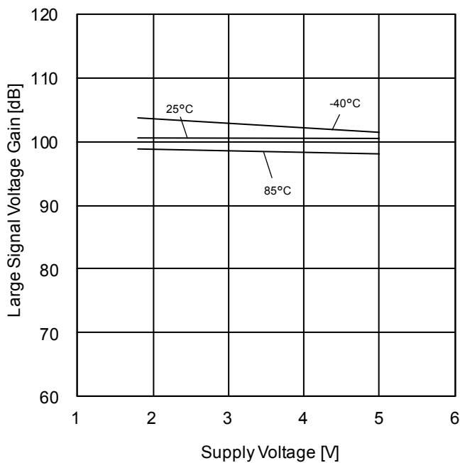
Figure 65. Large Signal Voltage Gain vs Supply Voltage ( R_L=2k\Omega )
