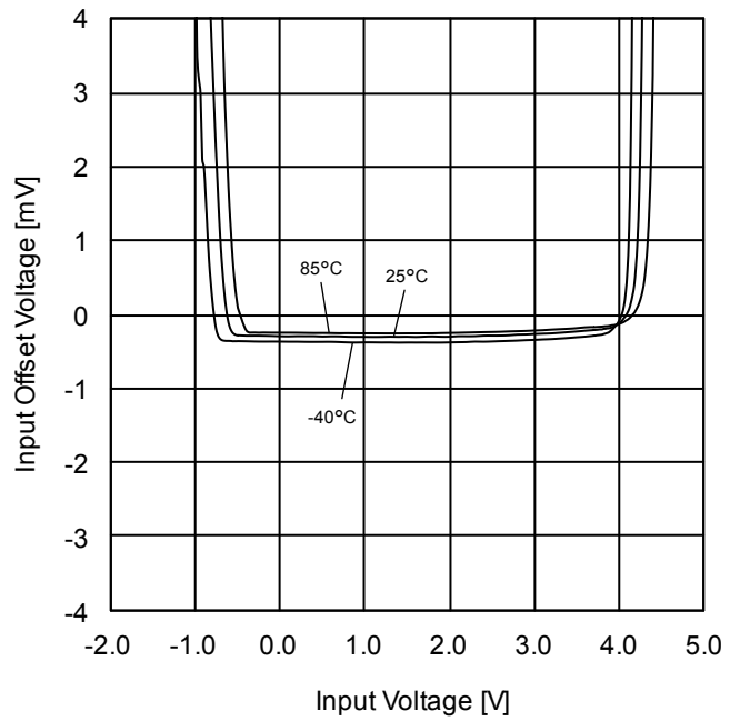
Figure 64. Input Offset Voltage vs Input Voltage ( V_{DD}=5V )
