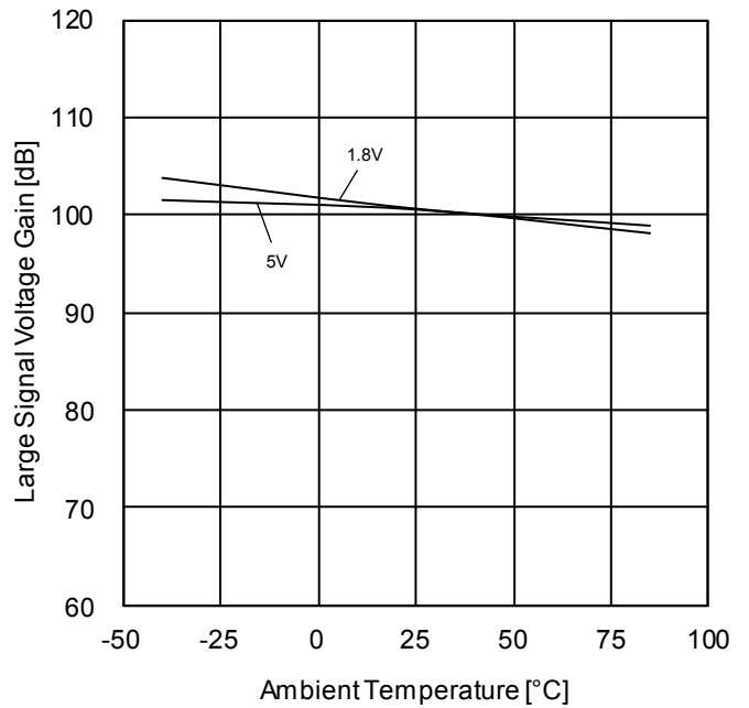
Figure 66. Large Signal Voltage Gain vs Ambient Temperature ( R_L=2k\Omega )
