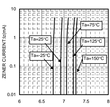
ZENER VOLTAGE : V_z(V) I_z - I_z CHARACTERISTICS
