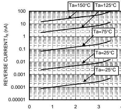
REVERSE VOLTAGE : V_R(V) I_r - V_R CHARACTERISTICS
