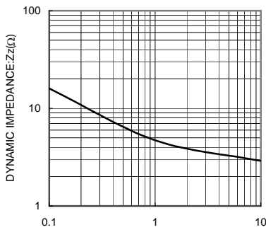
ZENER CURRENT( I_z ) Z_z - I_z CHARACTERISTICS
