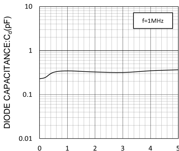
REVERSE VOLTAGE: Vr(V) V R -C d CHARACTERISTICS
