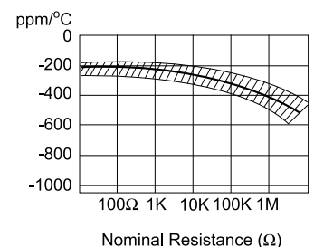
Temp. Coefficient
