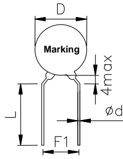
S Type (直线脚)
