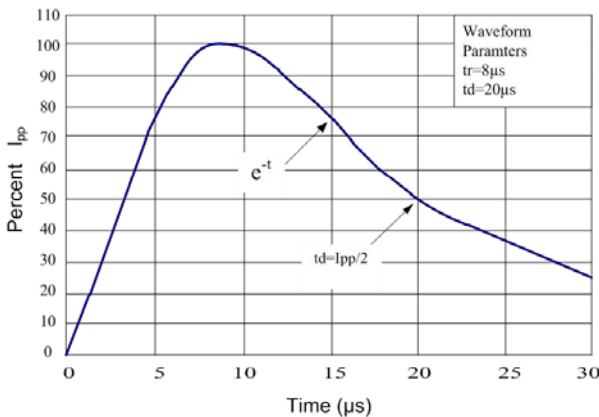
Figure 5: Pulse Waveform
