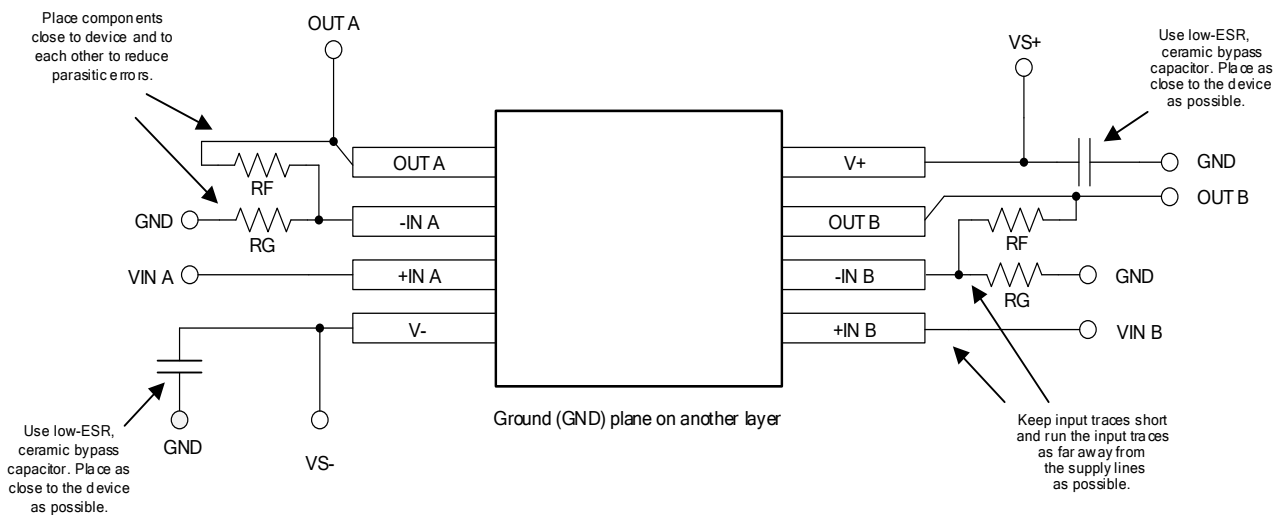
Figure 29. Layout Example
