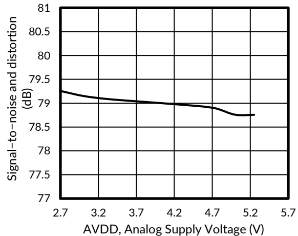
Figure 24. SINAD vs ANALOG SUPPLY VOLTAGE
