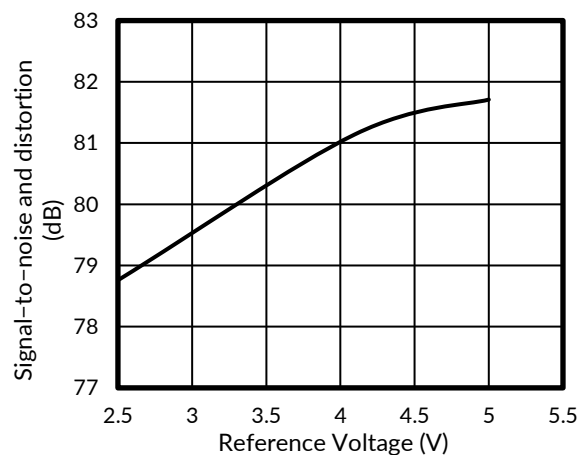
Figure 26. SINAD vs REFERENCE VOLTAGE
