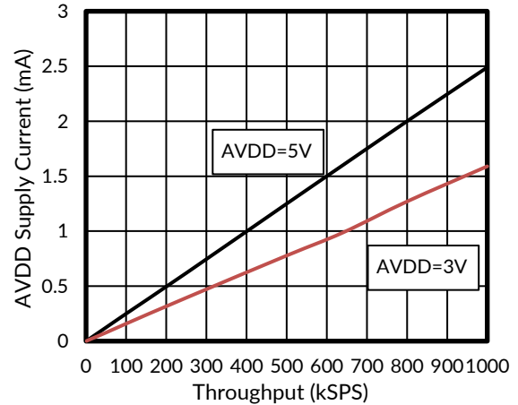
Figure 40. ANALOG SUPPLY CURRENT (Dynamic) vs SAMPLE RATE
