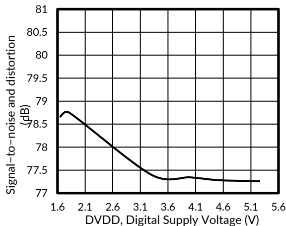
Figure 25. SINAD vs DIGITAL SUPPLY VOLTAGE
