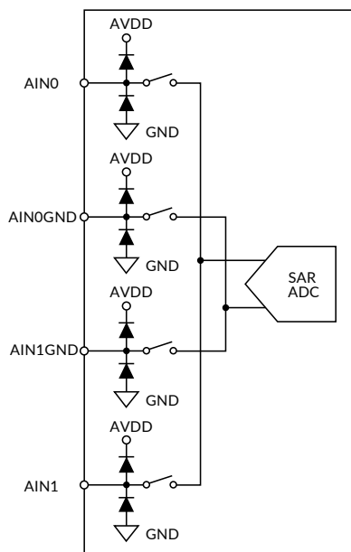
Figure 46. Analog Inputs
