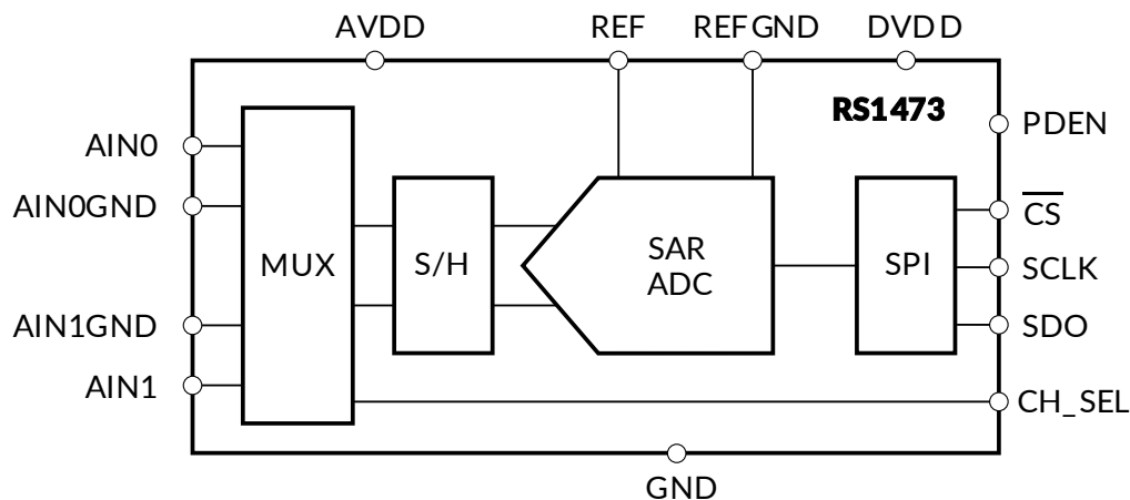
Figure 1. Block Diagram
