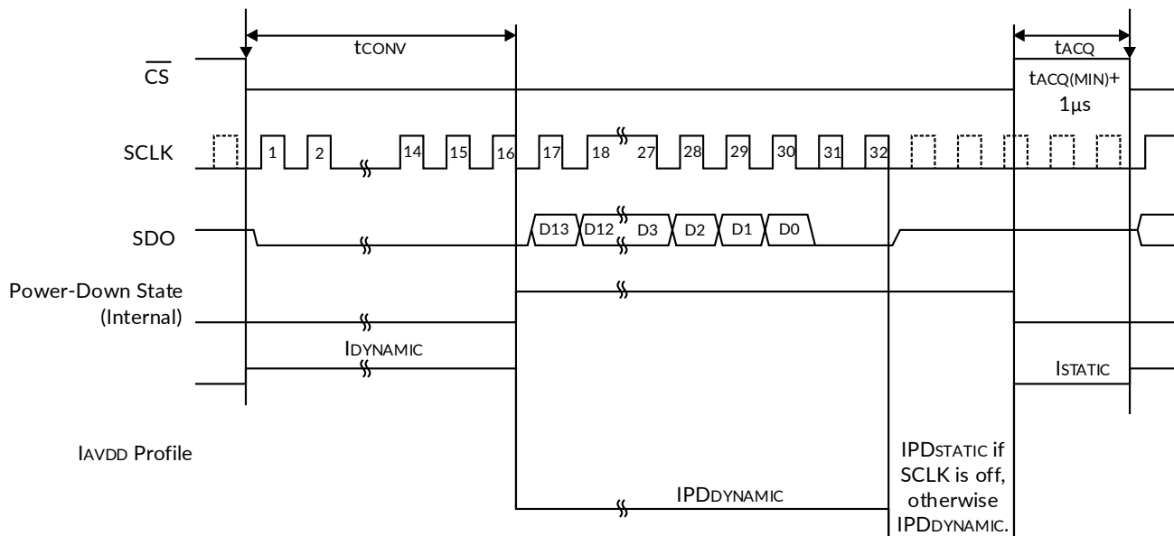
Figure 53. Power-Down Mode (PDEN = 1)
