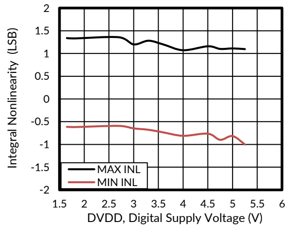
Figure 8. INL vs DIGITAL SUPPLY VOLTAGE
