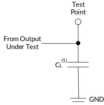
Figure 1. Load Circuit for Push-Pull Outputs
