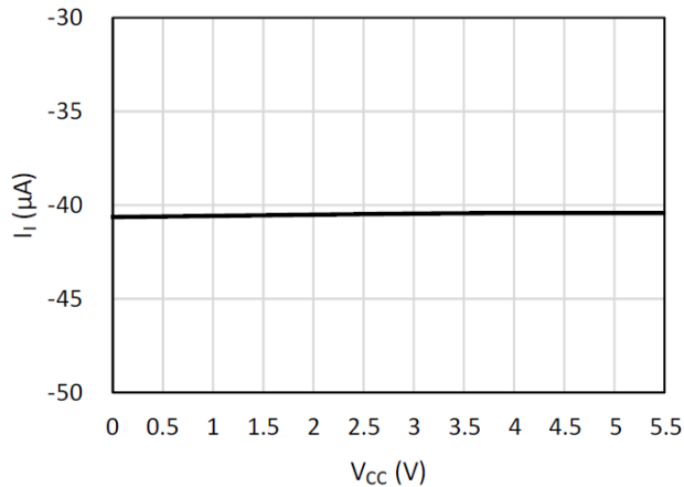
Figure 9. Bus Input Current vs. Supply Voltage, V_i=-7\text{V}
