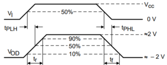
Figure 17 Measurement of Driver Differential Output Rise and Fall Times and Propagation Delays
