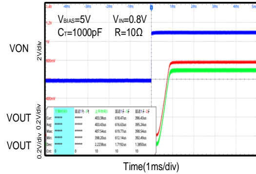
Figure 34. Turn-On Response Time
