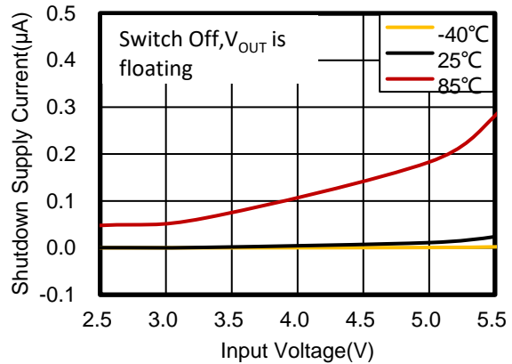
Figure 11. Shutdown Supply Current vs Input Voltage
