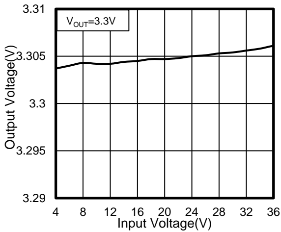
Figure 9. Line Regulation
