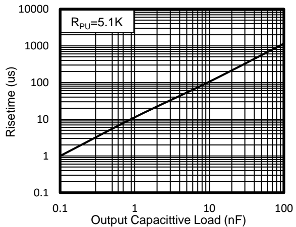
Figure 30. Risetime vs Capacitive Load
