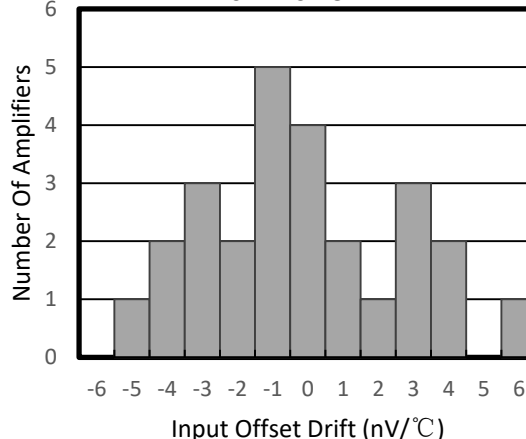
OFFSET VOLTAGE DRIFT PRODUCTION DISTRIBUTION
